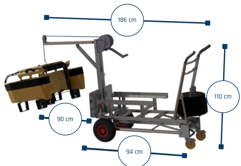
Figure b : Trolley unfolded setup
