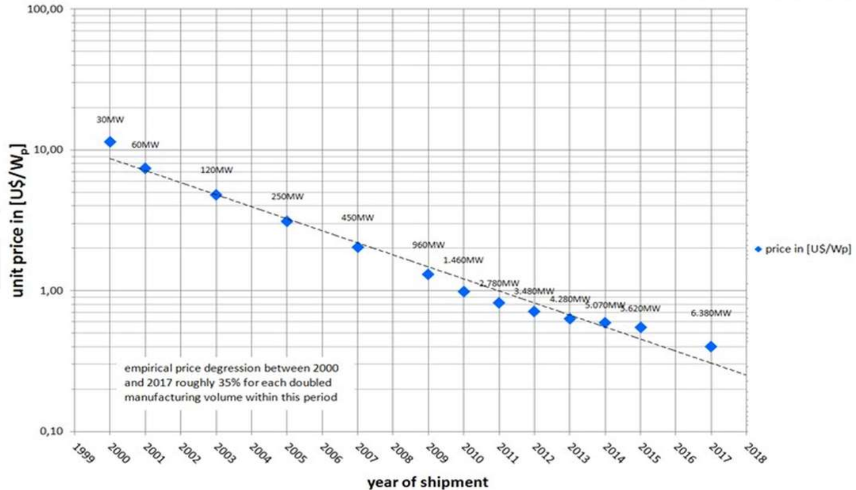
empirical learning curve a-Si:H cumulative shipment (*)
